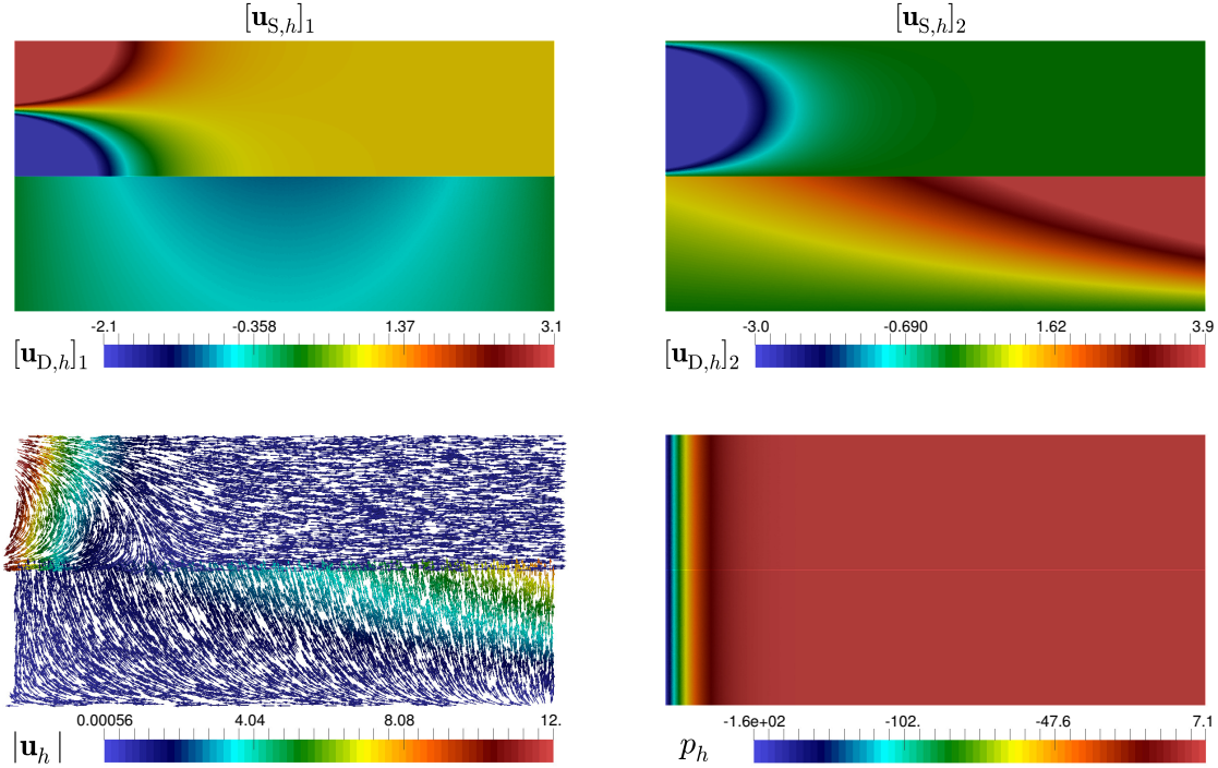
Figure 6.2: Example 2: Velocity components (top panels), velocity streamlines and pressure field in the whole domain (bottom panels).
