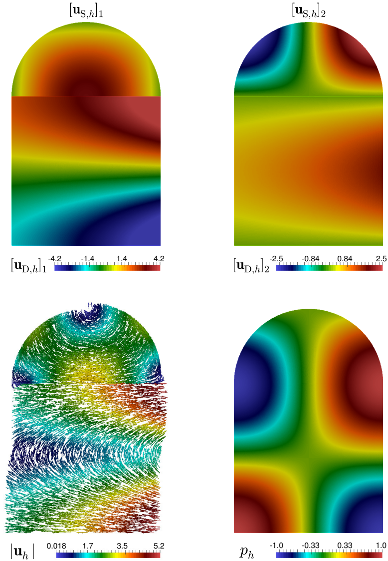
Figure 6.1: Example 1: Velocity components (top panels), velocity streamlines and pressure field in the whole domain (bottom panels).
