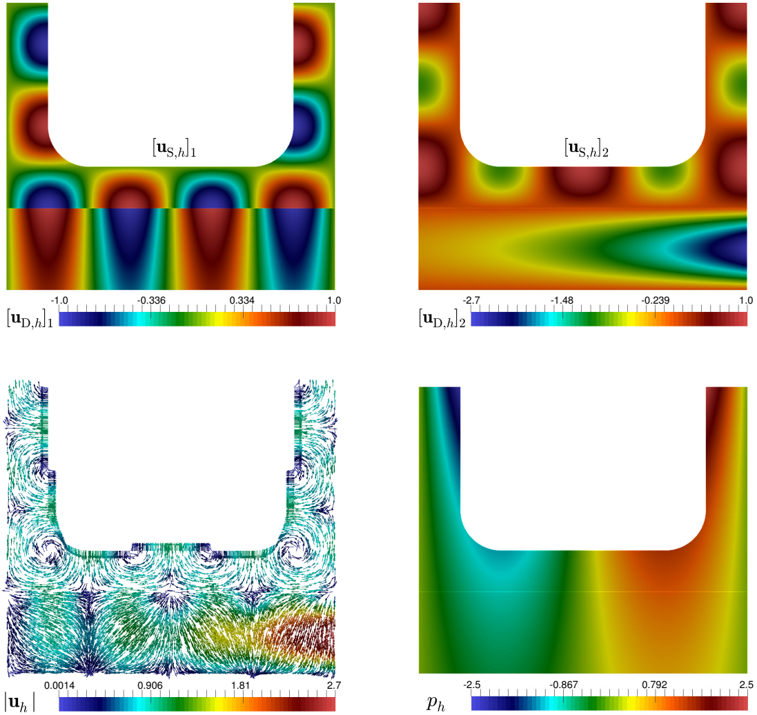
Figure 6.3: Example 3: Velocity components (top panels), velocity streamlines and pressure field in the whole domain (bottom panels).
