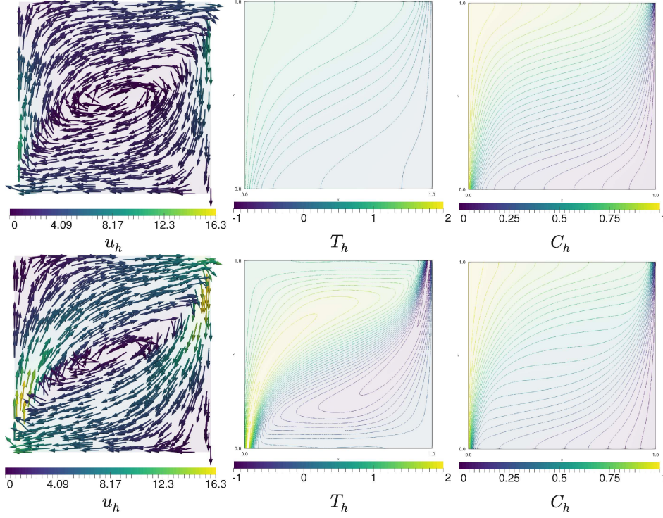
FIG. 5.1. Example 2 (porous cavity): (left) velocity field, (middle) isotherms and (right) concentration contours for (top) Du = 0.1 , (bottom) Du = 1 .
