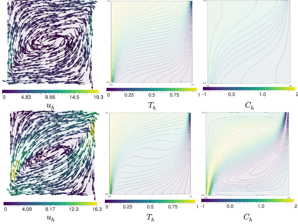
FIG. 5.2. Example 2 (porous cavity): (left) velocity field, (middle) isotherms and (right) concentration contours for (top) Sr = 0.1 , (bottom) Sr = 1 .
