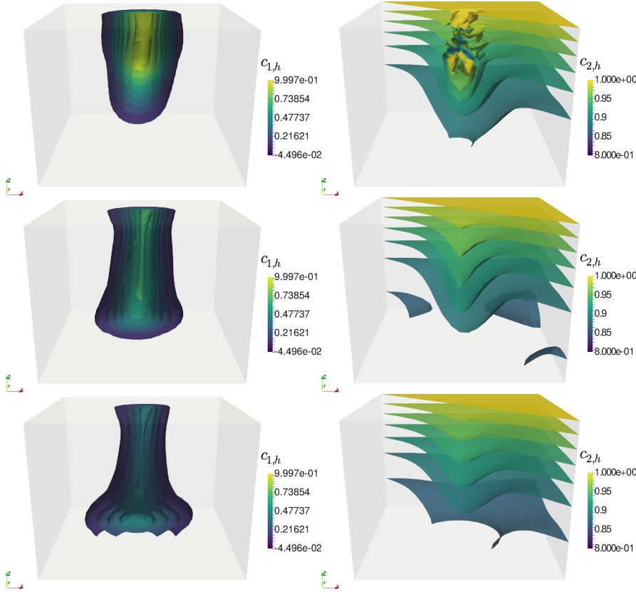
FIG. 5.4. Example 3 (bioconvection): patterns generated by the bacterial chemotaxis towards oxygen concentration. Snapshots of the obtained solutions at times (top) t = 0.1 , (middle) t = 0.3 and (bottom) t = 0.5 .
