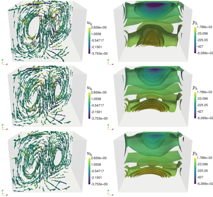
FIG. 5.5. Example 3 (bioconvection): patterns generated by the bacterial chemotaxis towards oxygen concentration. Snapshots of the obtained solutions at times (top) t = 0.1 , (middle) t = 0.3 and (bottom) t = 0.5 .
