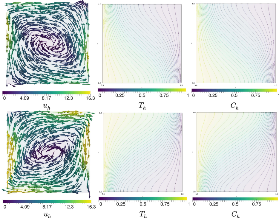
FIG. 5.3. Example 2 (porous cavity): (left) velocity field, (middle) isotherms and (right) concentration contours for (top) N = -5 , (bottom) N = 5 .
