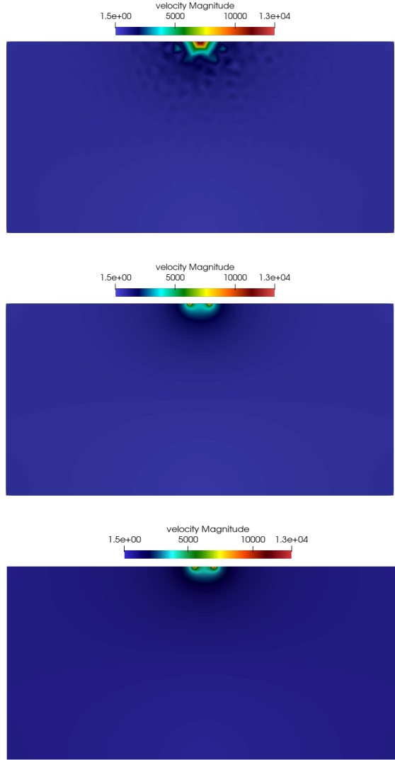
Figure 6: Isolines of the velocity magnitude using \mathbb{P}_1^2 \times \mathbb{P}_1 finite element spaces, corresponding to the solution with 1,286 elements on the initial mesh (top), the solution with 6,994 elements on the adapted mesh (middle) and the reference solution on a fine uniform mesh with 773,034 elements (bottom).
