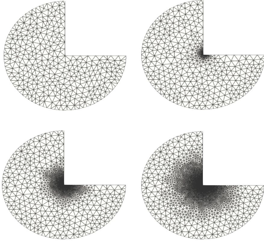
Figure 1: Suite of adaptive meshes: \mathcal{T}_{h,0} (top left), \mathcal{T}_{h,8} (top right), \mathcal{T}_{h,16} (bottom left) and \mathcal{T}_{h,20} (bottom right).
