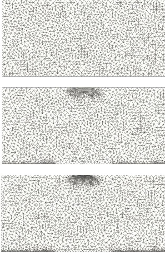
Figure 4: Suite of adaptive meshes: \mathcal{T}_{h,0} (top), \mathcal{T}_{h,2} (middle) and \mathcal{T}_{h,9} (bottom).
