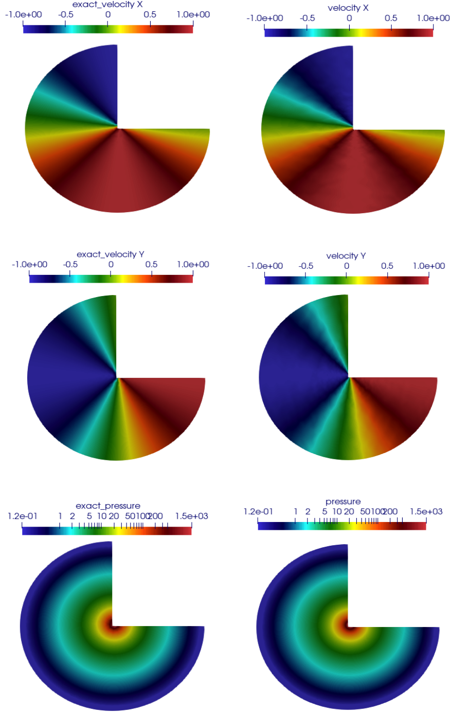
Figure 2: Components of the exact solution (left column) compared with the approximated solution (right column) obtained using \mathbb{P}_1^2 \times \mathbb{P}_1 on the final adapted mesh of 178,596 elements.
