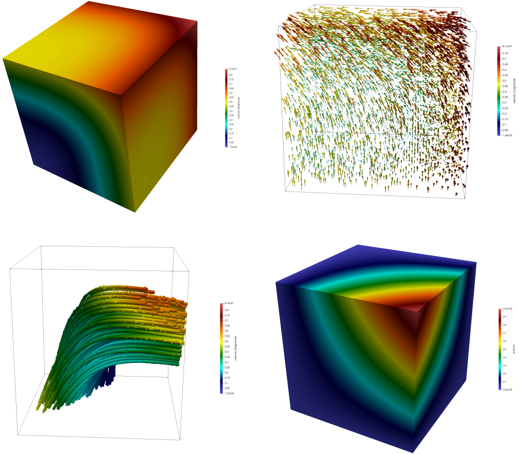
Figure 7: Approximated solution. Velocity magnitude (top left), velocity vectors (top right), velocity streamlines (bottom left) and isovalues of the pressure (bottom right). We use \mathbb{P}_1^3 \times \mathbb{P}_1 elements on a uniform mesh of 1,572,864 elements.
