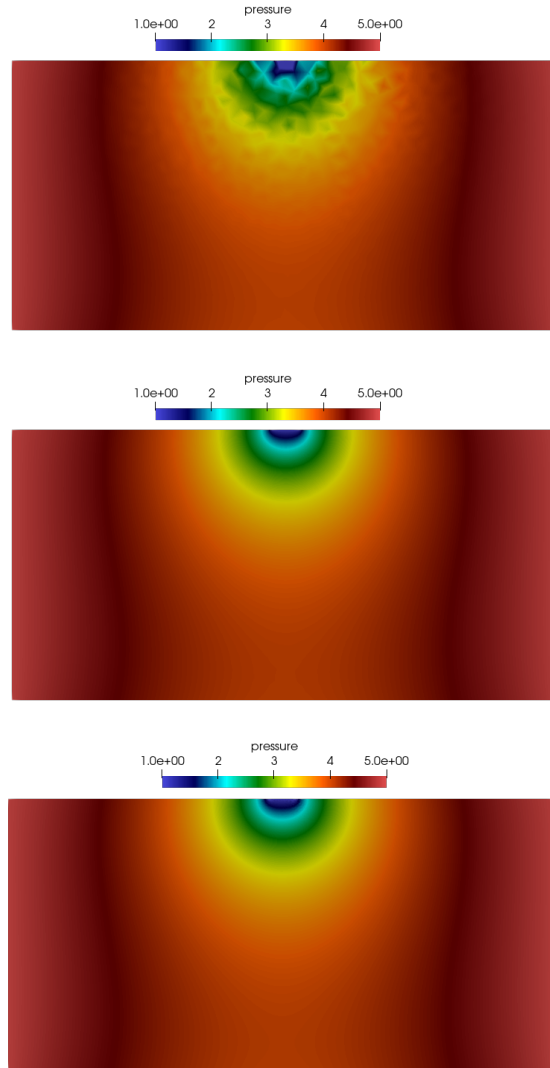
Figure 5: Isolines of the pressure using \mathbb{P}_1^2 \times \mathbb{P}_1 finite element spaces, corresponding to the solution with 1,286 elements on the initial mesh (top), the solution with 6,994 elements on the adapted mesh (middle) and the reference solution on a fine uniform mesh with 773,034 elements (bottom).
