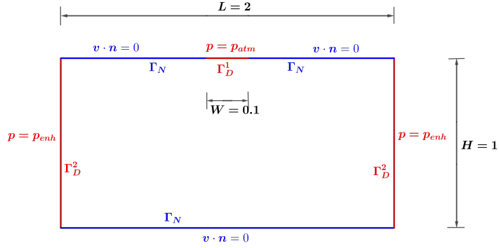
Figure 3: Sketch of \Omega with Dirichlet boundary conditions for the pressure in \Gamma_D^1 and \Gamma_D^2 , and normal trace zero for the velocity in \Gamma_N .
