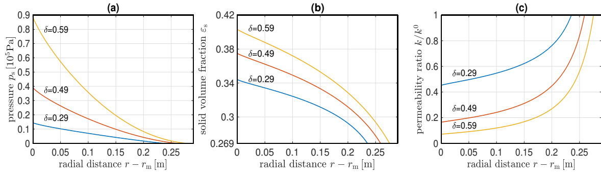
Fig. 8: Profiles of (a) p_s , (b) \varepsilon_s and (c) k/k^0 at simulated time t = 1800 s with the parameter values \delta = 0.29 , \delta = 0.49 , and \delta = 0.59 .
