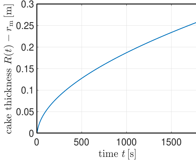
Fig. 4: Dynamics of sediment layer thickness on the filter surface.
